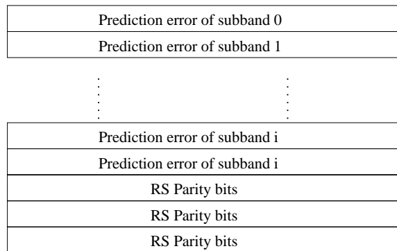
Figure 4: RS encoder of prediction error
