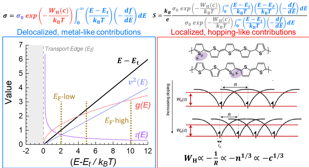
Figure 1: Summarizing the semi-localized transport (SLoT) model. The top row shows Eq. 1 and Eq.2 with the SLoT transport function (Eq. 3) evaluated in the integral expressions. Notably, \sigma is a function of all three terms, while S is only a function of the energy-dependent integral values. The leftmost blue box shows energy-dependent contributions, commonly found in delocalized and metal-like transport expressions. This plot shows that as the extent of doping increases, E_F increases with respect to the transport edge, E_t . Furthermore, the velocity squared of the carriers ( v^2 ), the density of states ( g(E) ), and the relaxation time \tau(E) , all vary as a function of doping. The product of these three terms is linear with respect to the x-axis, and therefore a linear transport function is used in the integrals. The rightmost red box shows energy-independent and localized contributions to the transport function. Poly(thiophene) chains can be oxidative doped, yielding polaronic charge carriers that are electrostatically attracted to the doping counterion ( A^- ). These polaronic charge carriers (represented by single barbed arrows) are localized in potential energy wells with depth W_H and separated by some distance R . In the above example, the carrier ratio is 2/10 or 0.2, representing two charge carriers for every ten aromatic ring sites. As the extent of doping increases, the distance between the carriers and the activation barrier decreases. At some carrier density ( n ) or carrier ratio ( c ), W_H \rightarrow 0 and the transport is thought to be delocalized. Figures adapted from Ref. 5.
