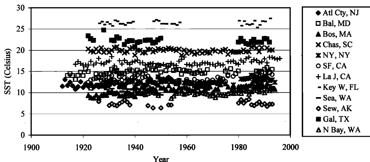
Figure 1. Time series of seawater temperatures from USA tide gauge sites.
