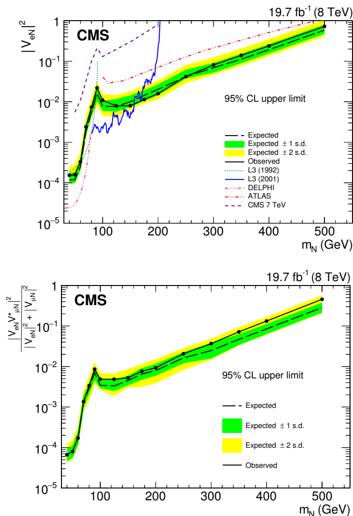
Figure 5. Exclusion region at 95% CL in the |V_{eN}|^2 vs. m_N plane (top) and |V_{eN}|^2 and |V_{eN}V_{\mu N}^*|/(|V_{eN}|^2 + |V_{\mu N}|^2) vs. m_N plane (bottom). The dashed black curve is the expected upper limit, with one and two standard-deviation bands shown in dark green and light yellow, respectively. The solid black curve is the observed upper limit. Also shown are the upper limits from other direct searches: L3 [22, 23], DELPHI [21], ATLAS [33], and the upper limits from the CMS \sqrt{s} = 7 TeV (2011) data [32].
