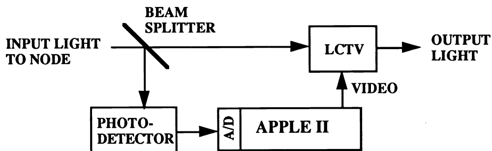
Figure 6. Block diagram of the EO neuron
