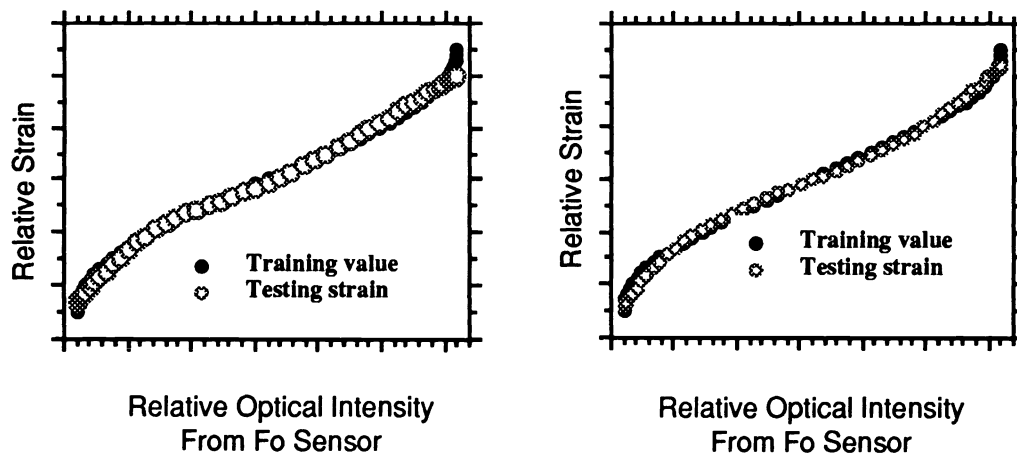
Figure 5.a Simulation results for 1/4/3 nodes RMS error/pattern = 2.82%.
