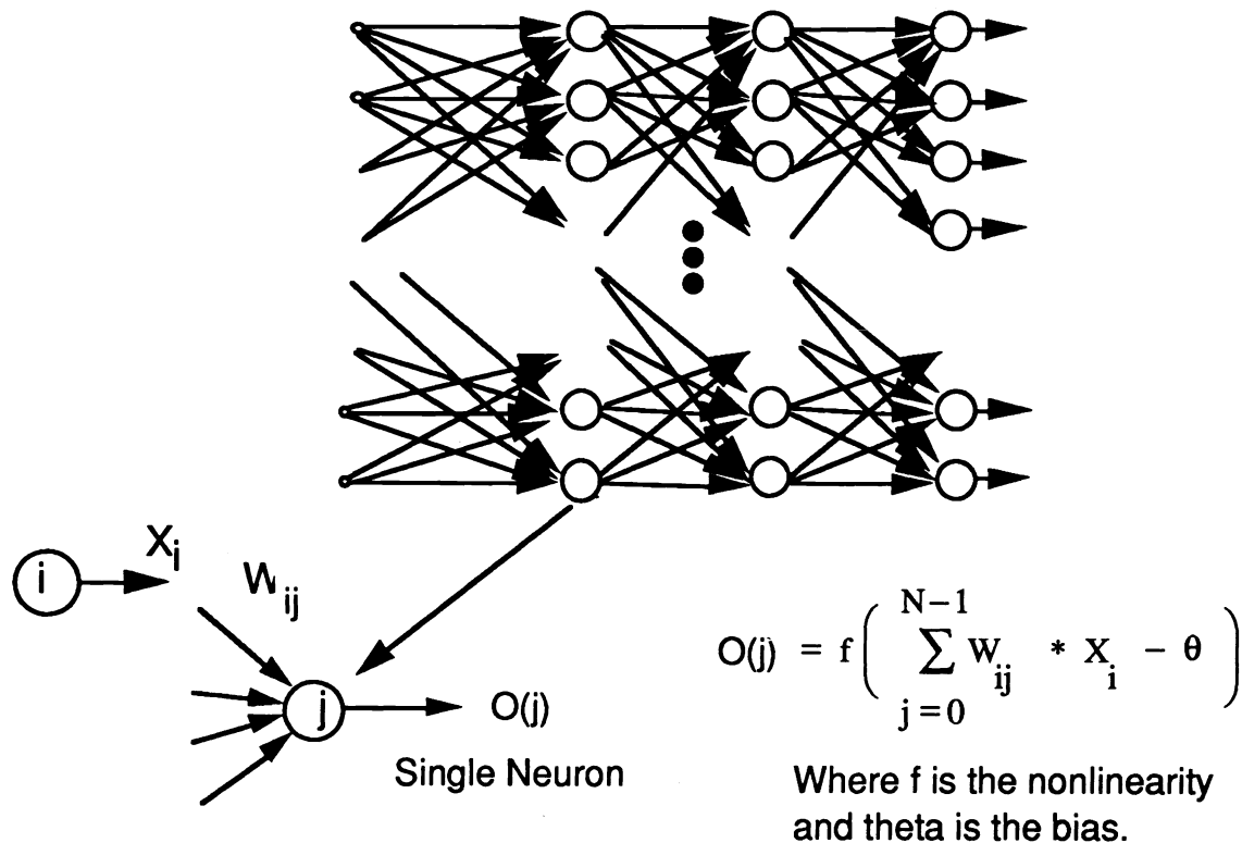
Figure 2. The training and use of artificial neural network processors for smart structures.
