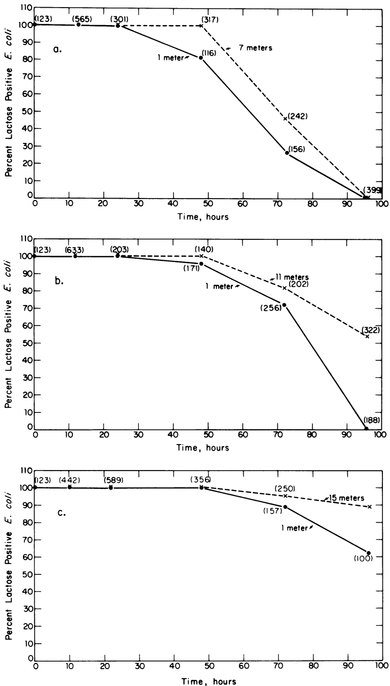
FIG. 2. Lactose changes of E. coli in Par Pond at station I (a) station II (b), and station V (c) when the reactor was operating. The numbers in parentheses represent the number of colonies replicated to eosin-methylene blue plates.
