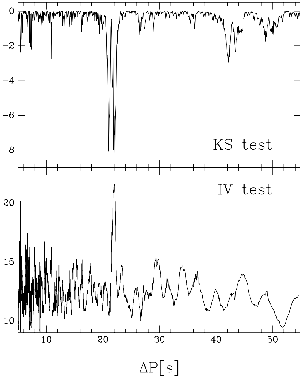
Fig. 10. The results of tests for period spacings. Upper panel: Kolmogorov-Smirnov (K-S) test; lower panel: Inverse Variance (IV) test. The K-S test shows a double minimum for period spacings \Delta P \approx 21 s and \Delta P \approx 22 s. The IV test shows a single maximum for a period spacing \Delta P \approx 22 s. The single peak points to a single \ell value being present, which we show to be \ell = 1 . We see no evidence of \ell = 2 modes, which should have a peak near 12.4 s.
