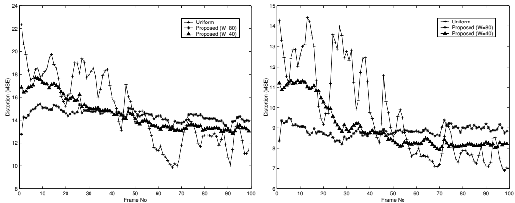
Figure 2. Distortion for adapting the L-FGS coded QCIF Akiyo sequence to CBR channels. Left: QCIF Akiyo at 48 kbps. Right: QCIF Akiyo at 80 kbps.
