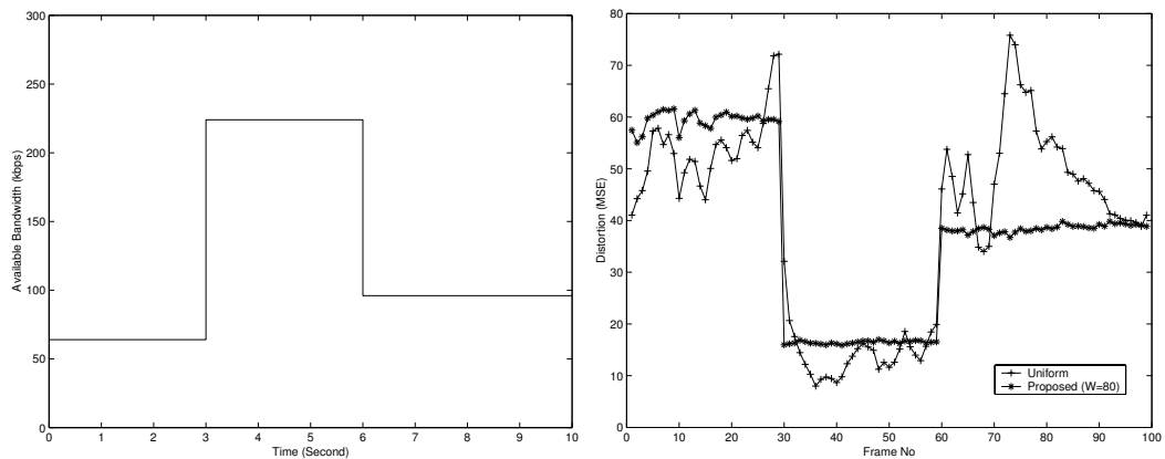
Figure 3. The simulation results for adapting the L-FGS coded Foreman sequence to the VBR channel. Left: Available bandwidth. Right: Distortion performance with window size=80.
