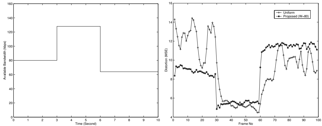
Figure 4. The simulation results for adapting the L-FGS coded Akiyo sequence to the VBR channel. Left: Available bandwidth. Right: Distortion performance with window size=80.
