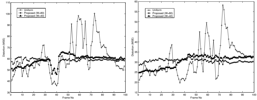
Figure 1. Distortion for adapting the L-FGS coded QCIF Foreman sequence to CBR channels. Left: QCIF Foreman at 64 kbps. Right: QCIF Foreman at 128 kbps.
