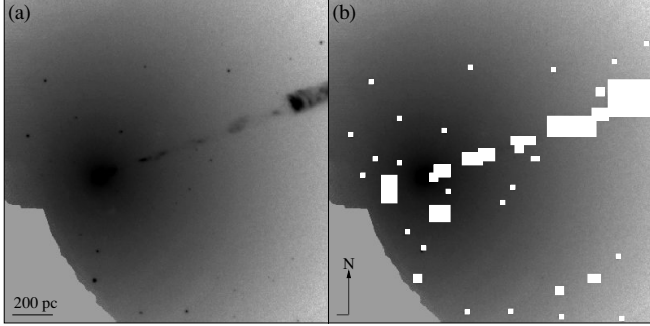
Figure 2. (a) ACS HRC F814W median combined image of M87 with a logarithmic stretch. (b) The mask overlaid on (a).
