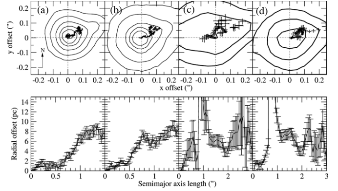
Figure 3. Top row: x and y ellipse centers overlaid on ACS contours. The point source is at (0,0). (a) and (b) HRC ellipse centers for SMA < 1''.5 . The jet (masked out for the fits) can be seen as an N–W extension. (c) and (d) WFC ellipse centers for SMA < 3''.0 . (a) and (c) F606W, (b) and (d) F814W. Bottom row: radial offsets of the ellipse centers.
