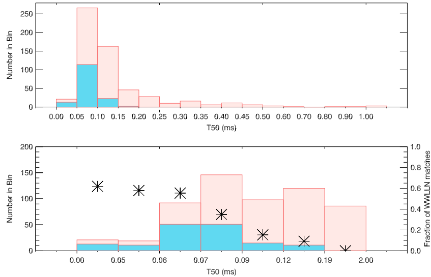
Figure 3. (top) The duration distribution in 50 \mu\text{s} time bins of the 594 TGFS (salmon) with the subset of 154 TGFS having a match with a simultaneous WWLLN discharge shown in blue. (bottom) We rebin the distributions such that each time bin contains at least 10n TGFS with associated simultaneous WWLLN discharges. The asterisks show the fraction of TGFS having WWLLN associations. Similar to Figure 2 but with the T_{50} s measured for counts detected above 300 keV. Compared to Figure 2, the width of the T_{50} values is narrower and peaked at lower values for those TGFS with WWLLN associations. The number of very short TGFS with associations is also higher, and the number of longer TGFS with associations lower than when the T_{50} values are measured using the entire GBM energy range.
