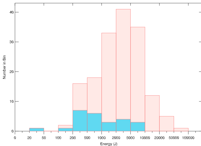
Figure 4. The estimated far-field VLF stroke energy of discharges measured by WWLLN in association with GBM-detected TGFs. Hutchins et al. [2012a] described the procedure and reliability of measuring energies associated with WWLLN discharges. We include here 164 WWLLN discharges associated with TGFs for which energy measurements are available, and which have uncertainties lower than 70% of their value. The subset of nonsimultaneous associations, which are farther than \pm 200 \mu\text{s} from the TGF peak, is shown in blue, the simultaneous associations in salmon. The nonsimultaneous discharges have a significantly lower median energy (700 J) than the simultaneous discharges (3.1 kJ).
