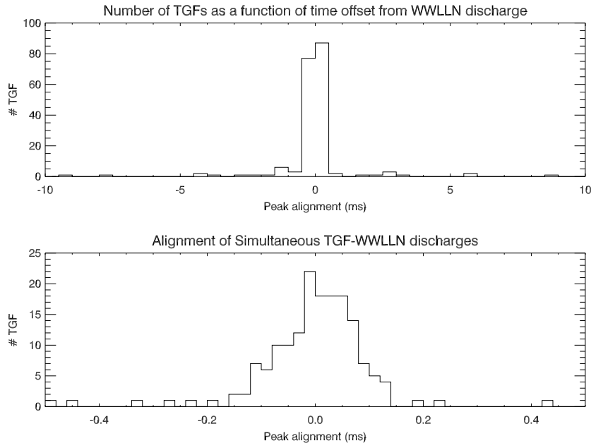
Figure 1. (top) Offset distribution, in 500 \mu\text{s} bins, of the TGF peak—the midpoint of the T_{50} interval (see text)—from 186 matched discharge times of group arrival measured by WWLLN. (bottom) Zoom in on the region close to the TGF peak, containing most of the GBM-WWLLN matches. A 400 \mu\text{s} interval centered on the TGF peak is used to define GBM-WWLLN simultaneity, and contains 154 of the associations.
