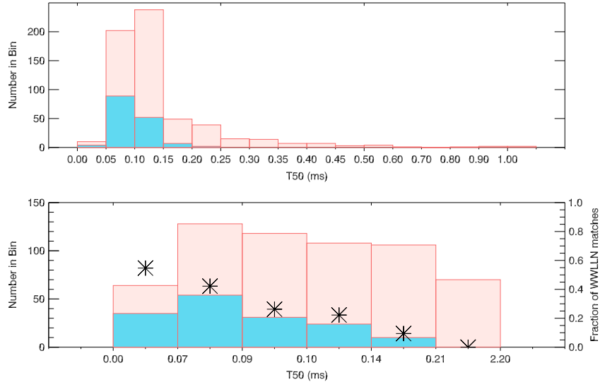
Figure 2. (top) The duration distribution in 50 \mu\text{s} time bins of the 594 TGFs (salmon) with the subset of 154 TGFs having a match with a simultaneous WWLLN discharge shown in blue. We exclude likely electron-beam TGFs, which are generally much longer than the TGFs detected in gamma rays [Briggs et al. , 2011], and suppress for display purposes the two likely gamma ray TGFs that have durations longer than 1 ms. (bottom) We rebin the distributions such that each time bin contains at least 10 TGFs with associated simultaneous WWLLN discharges (the final large bin has no matches in the WWLLN data). The asterisks show the fraction of TGFs having WWLLN associations.
