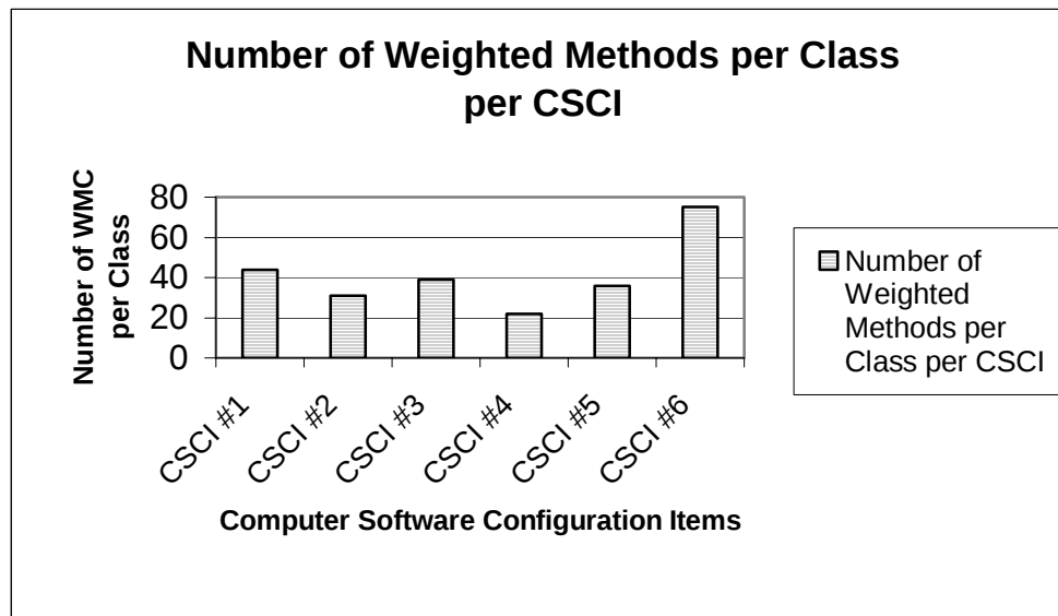
Figure 5-12 CSCI Weighted Methods per Class Data
