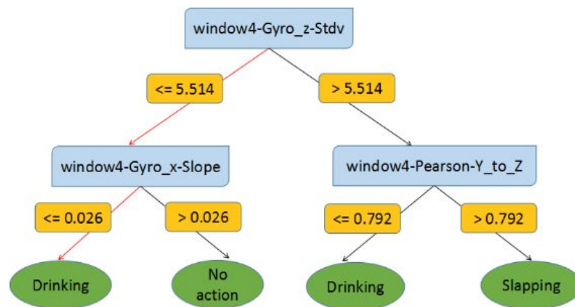
Figure 3.5 — The blue block is the feature. The yellow block is the value of each feature. The green circle is the leaf node represents the class
