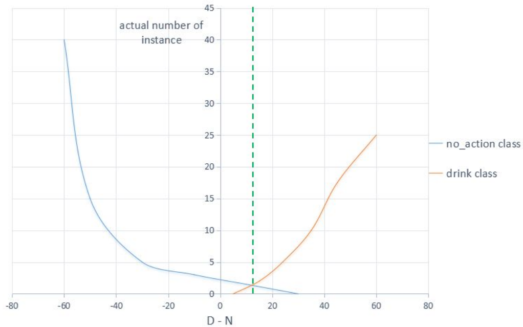
Figure 3.7 — The green dash line is the threshold
