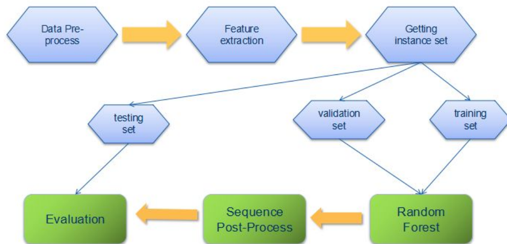
Figure 3.1 — The basic components of the overall systems.
